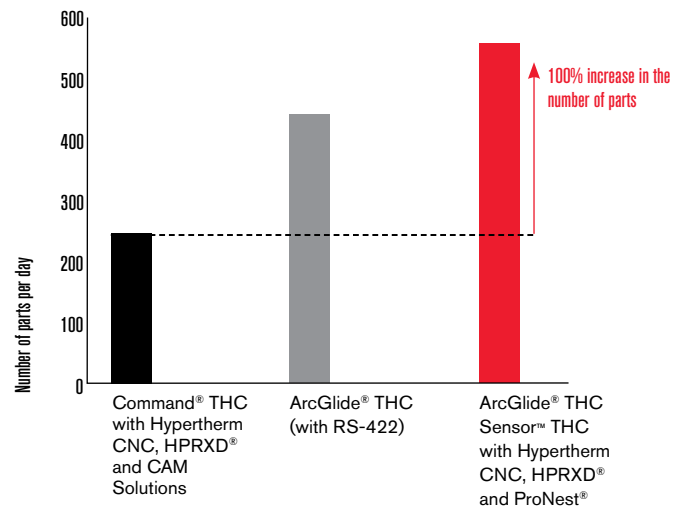
Number of parts - 203 mm (8") flange
